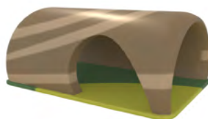
log crawl
